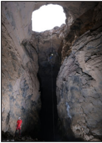
fig. 27: Shaft of warm puka 7; picture by B. Langford).
