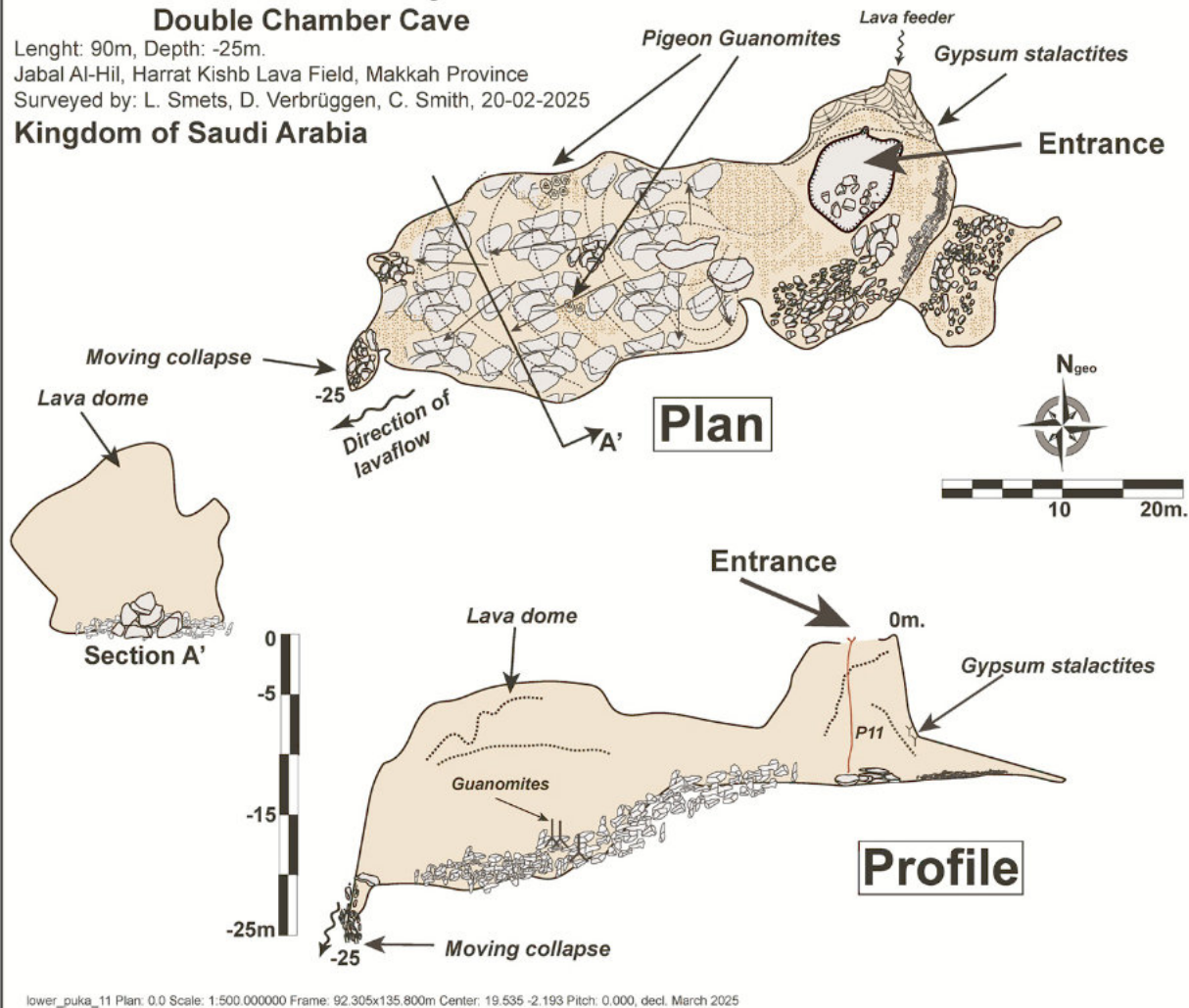
fig. 38a Survey of Double Chamber Cave
