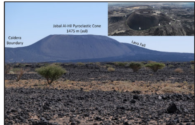
fig. 3: View on Jabal Al-Hil volcano; picture by B. Langford
