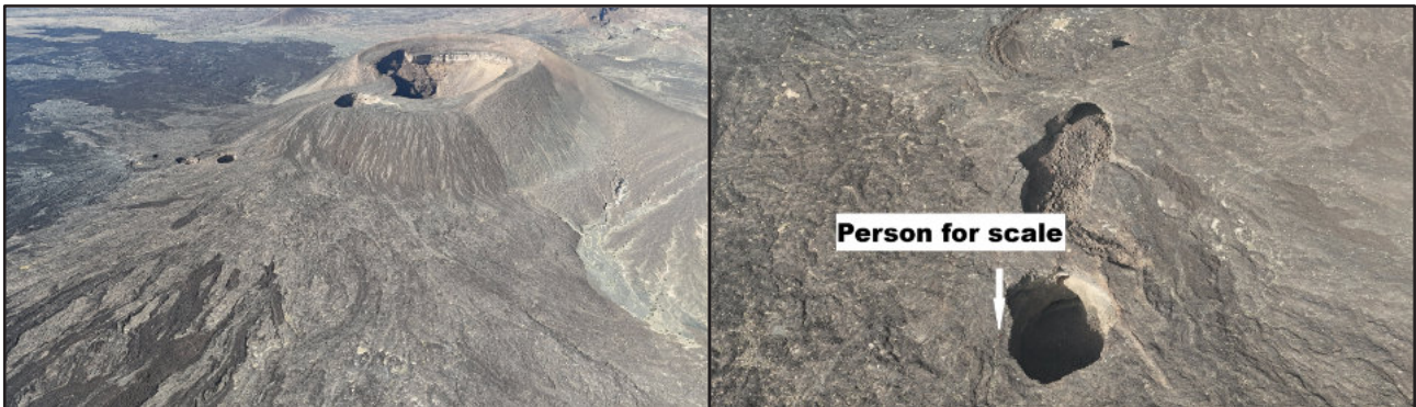
fig. 47c: Left, The Jabal Al-Hil Volcano;
