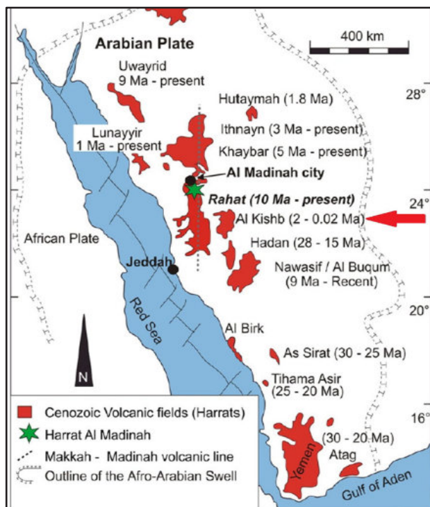
Fig 2: Lava fields of the Arab peninsula (red patches).
