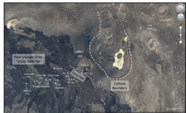
fig. 4: View on the Jabal Al-Hil Southwest Lava flow, the location of our Basecamp and the First Cave. Google Earth rendering by B. Langford
